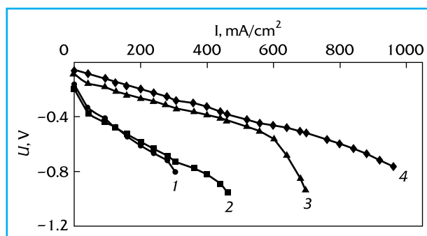
Current-voltage characteristics of oxygen electrodes with the active layer made of various electrode materials: 1 — PUMLCNT \Theta = 50\% ; 2 — \text{g-C}_3\text{N}_4 ; 3 — composite \text{C}_3\text{N}_4 with PUMLCNT \Theta = 50\% ; 4 — PUMLCNT with applied Pt in the amount of 10 mass % and \Theta = 50\%
