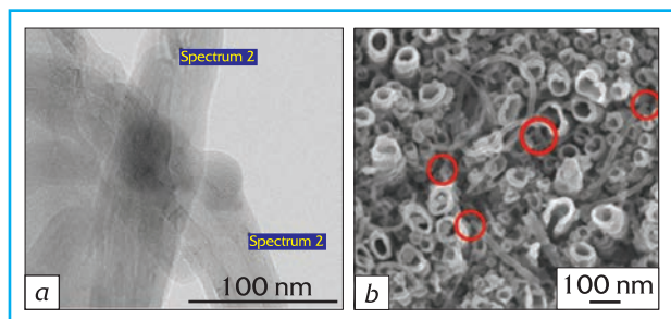
Microphotographs of the composite with partially unzipped multilayered carbon tubes and \text{g-C}_3\text{N}_4 (a) and \text{NT-TiO}_2/\text{PUMLCNT} (b), \Theta = 50\% , where red circles show \text{TiO}_2 -introduced PUMLCNT \Theta = 40\%
