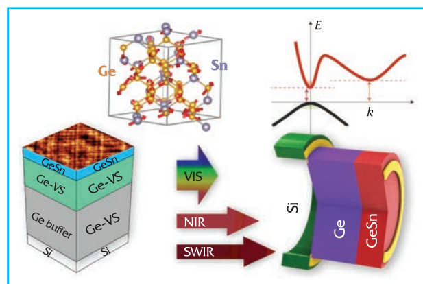
Schematic image of semiconductor structure of the wide-band sensor based on GeSn alloys
