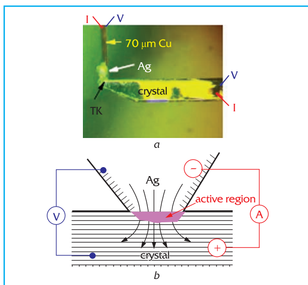
Photograph of point contact (PC) between the specimen and silver (a). Model of PC between the tip and Ag tip, where shown in red is the "region" of the maximum electric field concentration (b). The arrows show current propagation in PC
