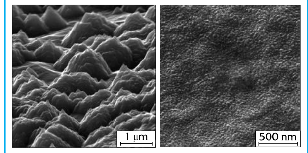
SEM microphotographs of the hierarchic submicron structure with nano-sized relief of the barrel bore surface (left) and of the dense surface after fabricating the film of nanocluster formations on the structured surface by trampoline sputtering of a target
