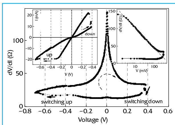
Differential resistance dV/dI and BAX (left-hand insert) of PC between Cu_xTiSe_2 specimen and silver electrode at "helium" temperature 4K. The right-hand window shows the "logarithmic" behavior of dV/dI
