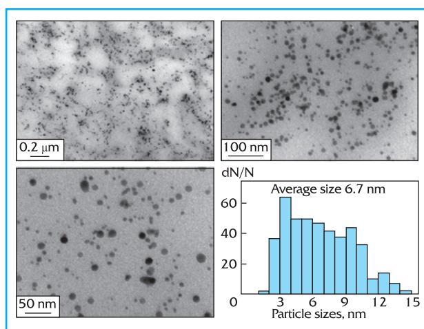
Electron microscopy images and histogram of silver nanoparticles distribution in the biopolymer nanocomposite produced by thermochemical reduction of \text{Ag}^+ ions
