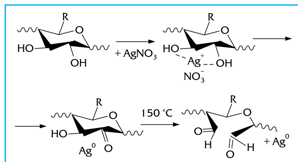
Mechanism of thermochemical reduction of \text{Ag}^+ ions in biopolymer nanocomposite
