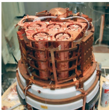
Assemblies with lithium molybdate crystals, mounted in ultra-low background cryostat in Modan underground laboratory in France
