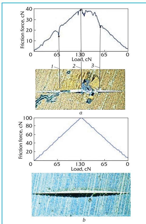
Results of diamond indenter scanning of the film sputtered without preliminary submicron- and nano-size surface structuring (a) and after it (b)
