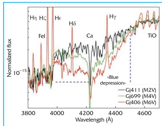
Spectra of M dwarfs GJ411 (M2), GJ699 (M4), and GJ406 (M6) from the Sun's vicinity, which demonstrate blue depression in the 4000—4500 \text{\AA} wave range. Hydrogen emission lines can be seen in the spectrum of GJ406, which suggests a relatively young age of the star
