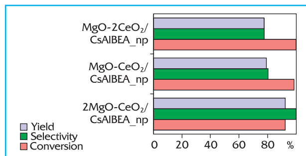
Catalytic characteristics of MgO-CeO 2 /CsAlBEA nanocomposites, depending on Mg/Ce ratio
